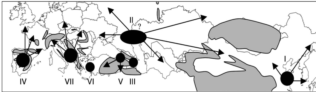
Fig. 5. Potential refuges (black), barriers (grey), and range expansion (arrows) of the seven clades.
