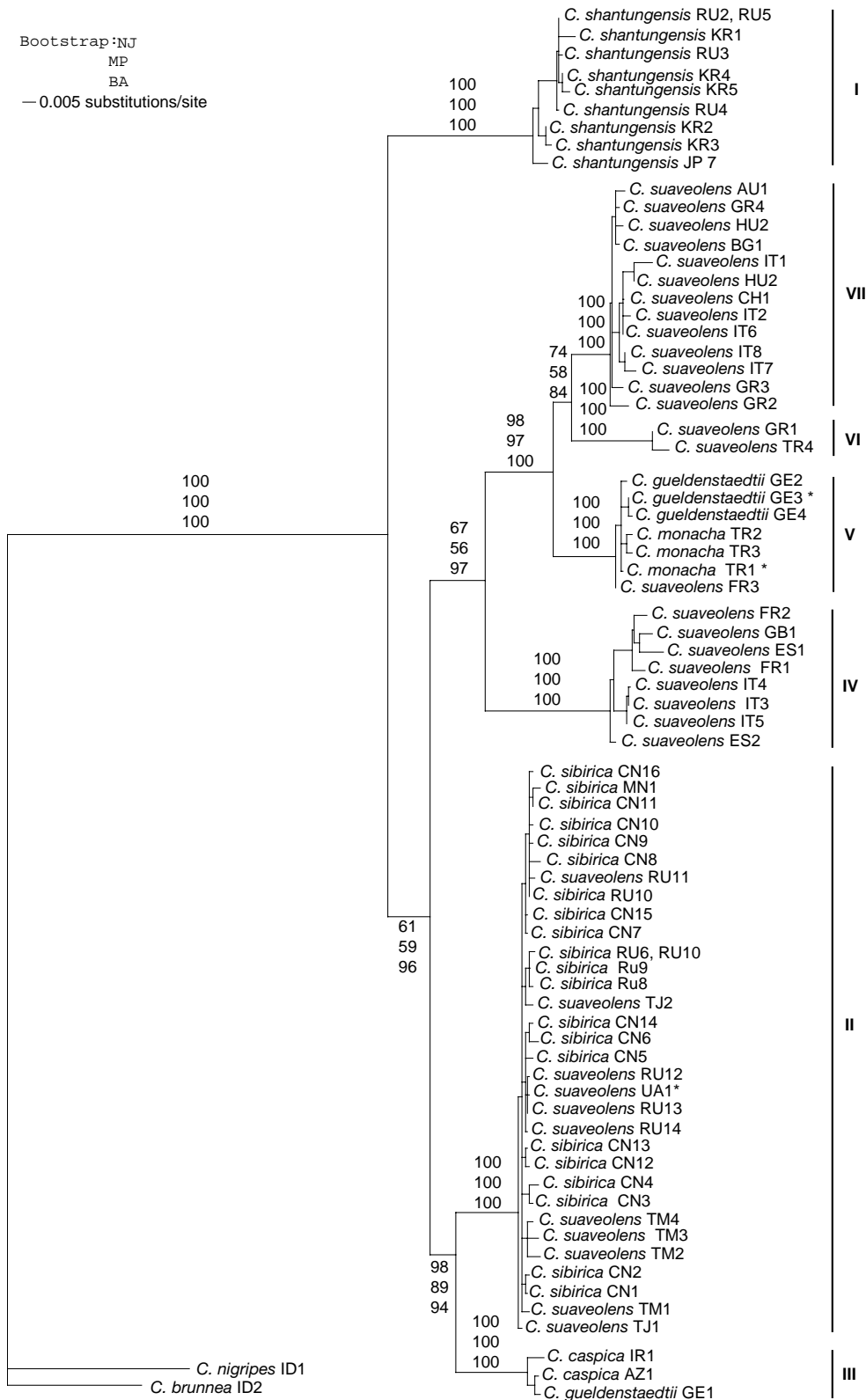
Fig. 2. Phylogeny of the 998 bp cyt-b fragment analysed with maximum likelihood, using the TVM + G model of substitution and TBR branch swapping. Values in branches are bootstrap indices of support for the major branches for Bayesian (BA), parsimony (MP), and distance (NJ) analyses (percentage of 1000 replications for each of the 10 random orders of stepwise addition of sequences). Codes are as in Table 1.
