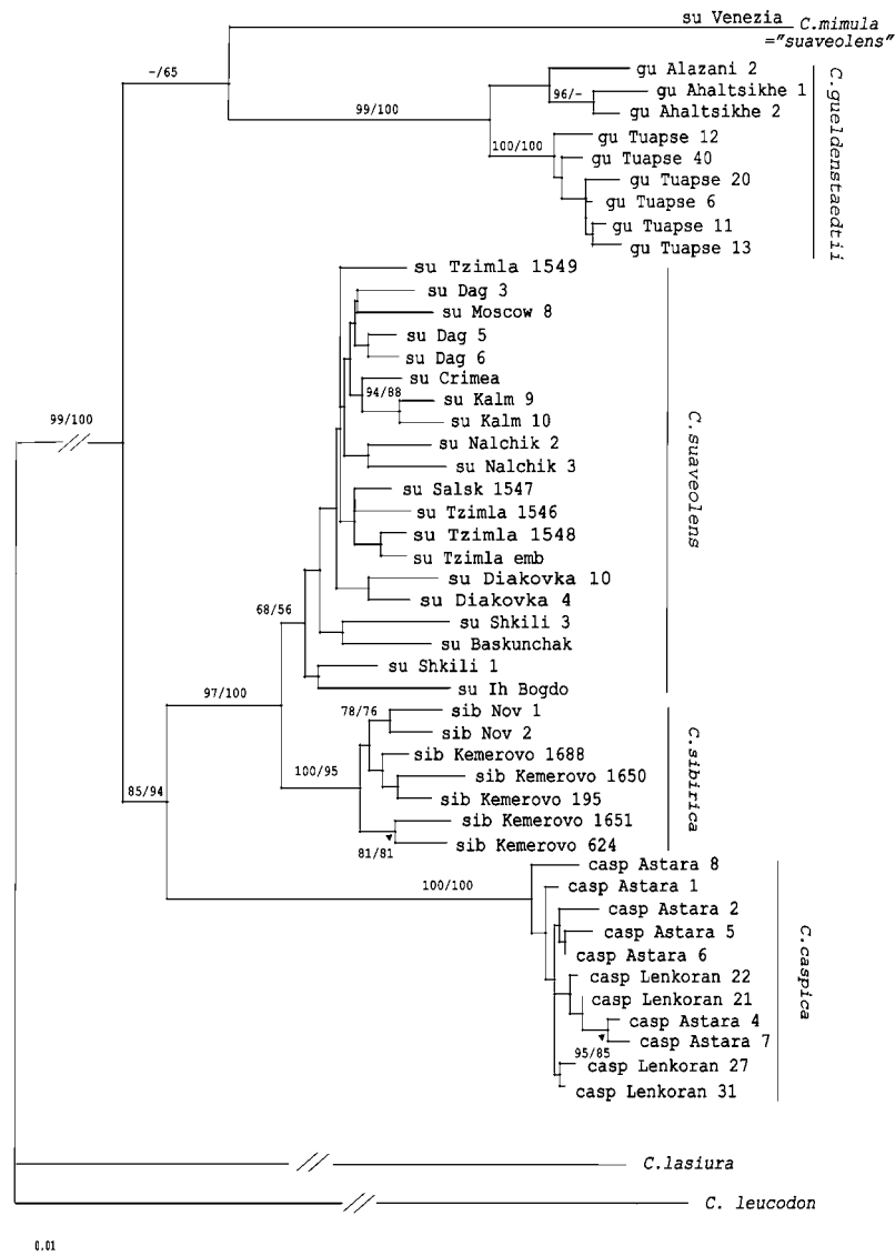
Figure 4 NJ tree of the relationships of the Crocidura suaveolens species group inferred from the Nei-Li genetic distances based on the combined results of inter-MIR- and inter-SOR-PCR. The designations are as in Figures 2 and 3.
