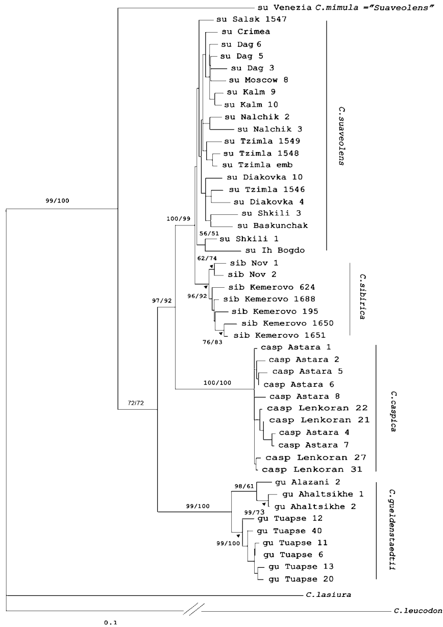
Figure 3 NJ tree of the relationships of the Crocidura suaveolens species group inferred from the Nei-Li genetic distances based on the results of inter-MIR-PCR. The designations are as in Figure 2.
