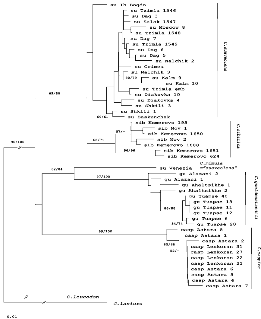
Figure 2 NJ tree of the relationships of the Crocidura suaveolens species group inferred from the Nei-Li genetic distances based on the results of inter-SOR-PCR. The bootstrap values ( bv \geq 50\% ) obtained from 1000 replications in NJ and MP analysis are given above the branches (NJ/MP). C. lasiura and C. leucodon are used as an outgroup.
