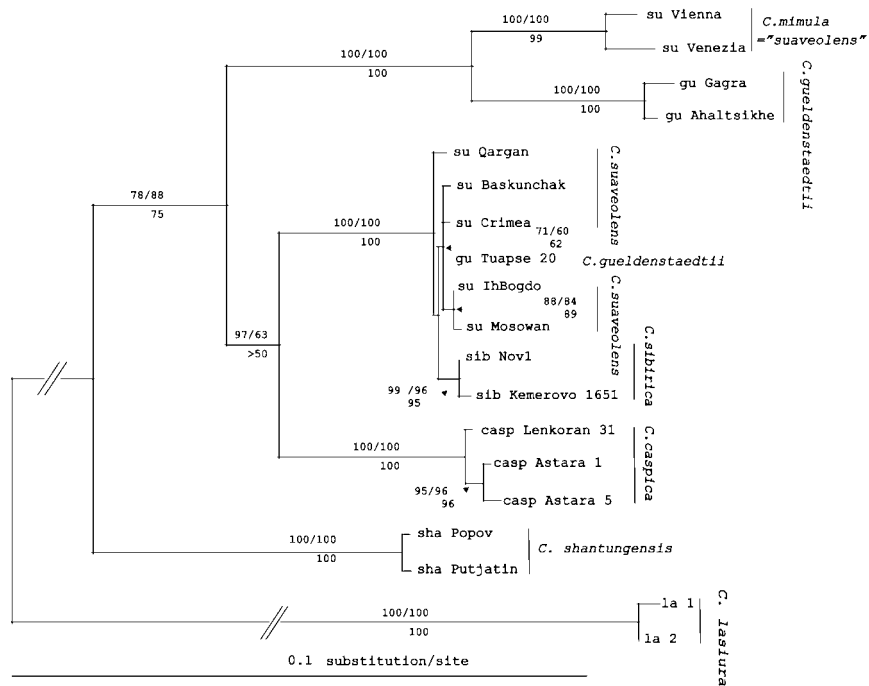
Figure 5 ML tree generated using a TrN+G+I model of the Crocidura suaveolens species group based on near-complete mitochondrial cytochrome b sequences. Bootstrap values \geq 50\% obtained from 100 replications are given above the branches (NJ/MP) for NJ and MP analyses and below branches for ML analysis (100 replicates). C. lasiura is used as an outgroup.
